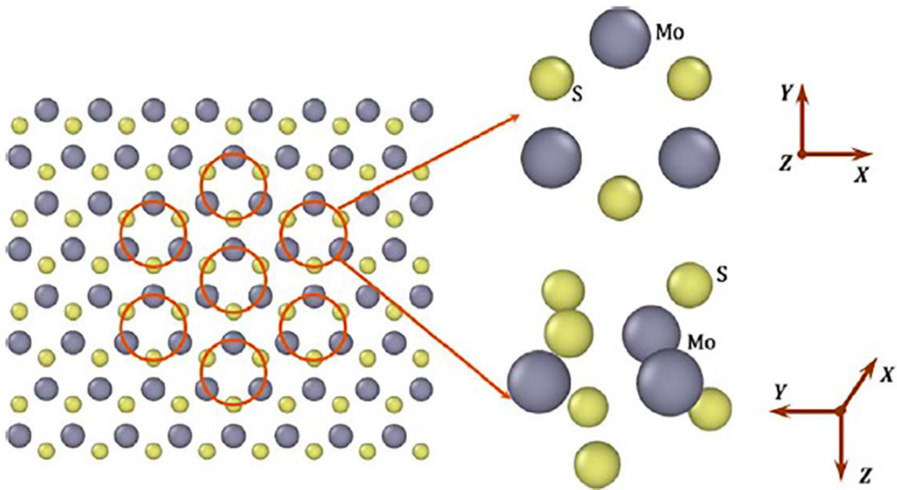
Fig. 3. Grains in \text{MoS}_2 lattice.
